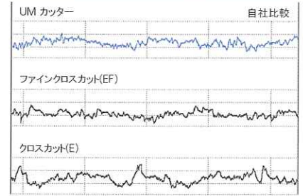
Comparative diagram of the surface quality (Roughness μm)
